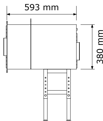
SIDE ELEVATION
